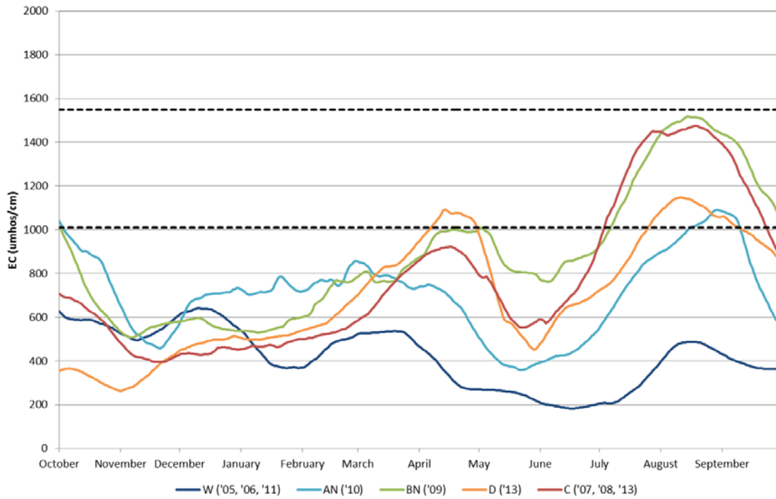
Crows Landing mean 30-day running average "Planned" EC by Water Year Type (Oct. 1, 2005 - Sept. 30, 2013)
