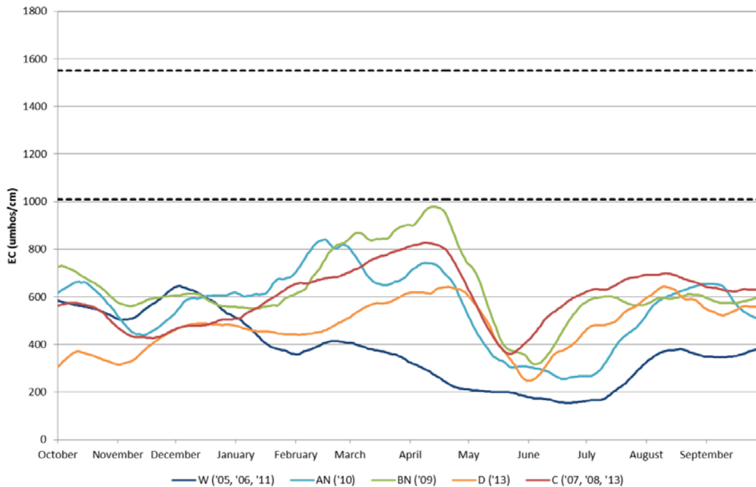
Maze Road mean 30-day running average "Planned" EC by Water Year Type (Oct. 1, 2005 - Sept. 30, 2013)
