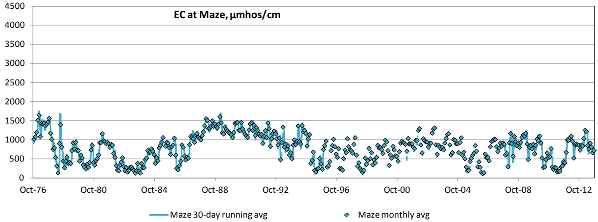
Oct 1976-2013 Monthly average EC at Maze (points) + daily 30 day running average (line w/out points)
