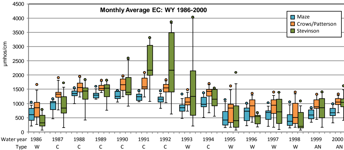
WY 1986 - 2000 Observed monthly average EC at Maze, Crows/Patterson, Stevinson by WY
