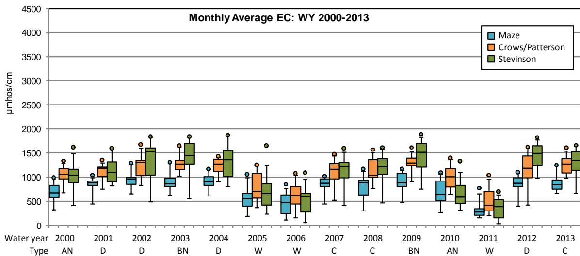
WY 2000 - 2013 Observed monthly average EC at Maze, Crows/Patterson, Stevinson by WY
