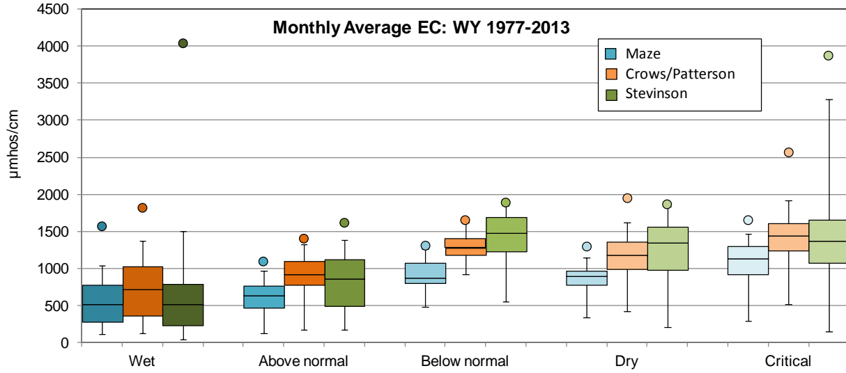
WY 1977-2013 EC at Maze, Crows/Patterson, Stevinson by WY type (e.g. W, AN, BN, D, C)
