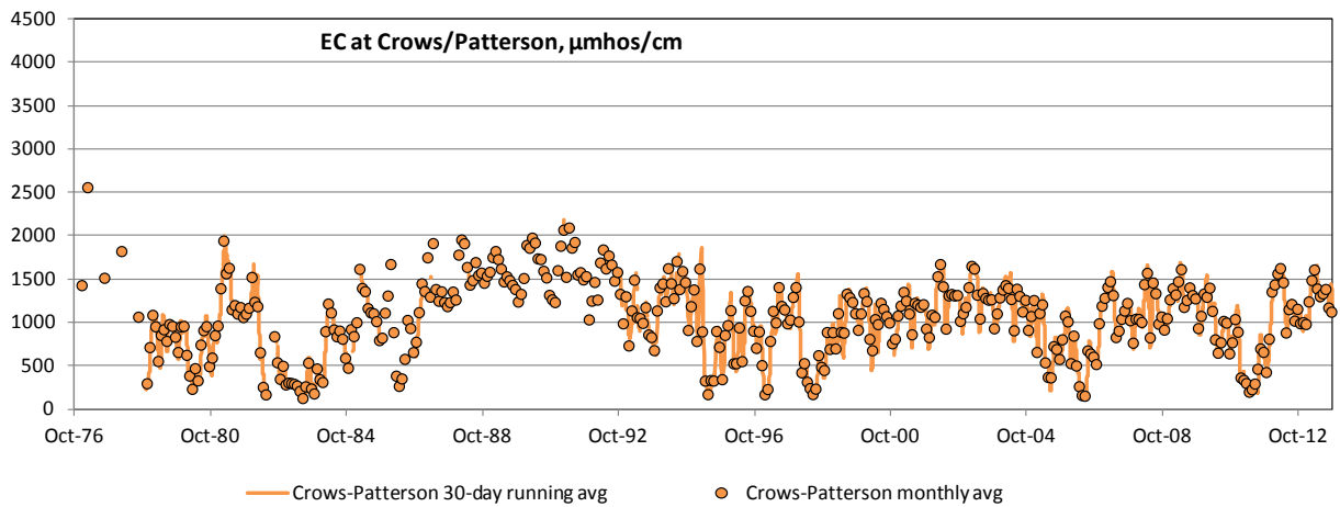
Oct 1976-2013 Monthly average EC at Crows/Patterson (points)+ daily 30 day running average (line w/out points)
