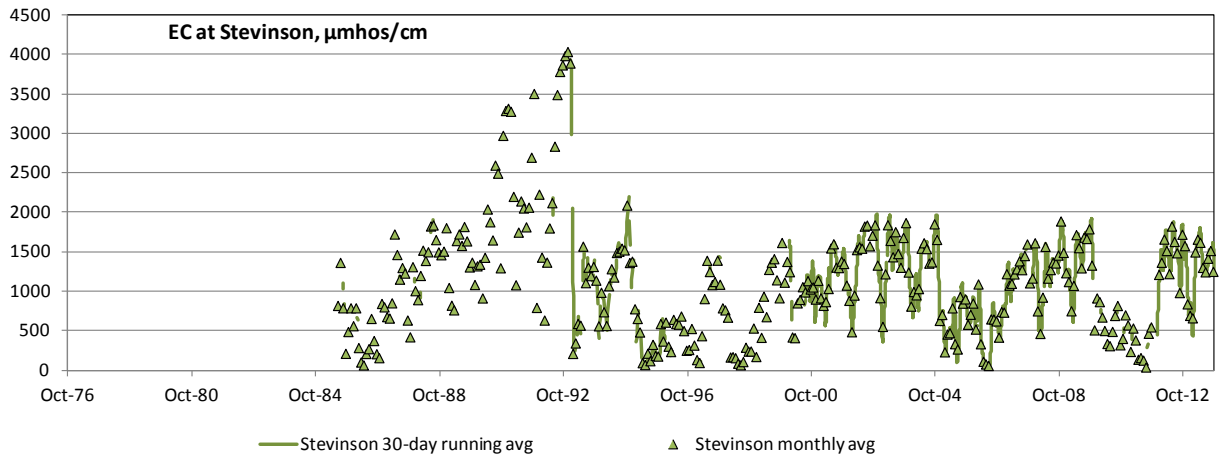
Oct 1976-2013 Monthly average EC at Stevinson (points) + daily 30 day running average (line w/out points)
