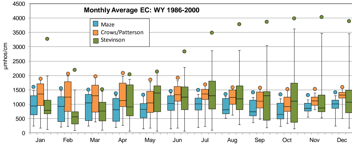
WY 1986 –2000 Monthly average EC by month (Jan, Feb, Mar,...) at Maze, Crows/Patterson, Stevinson
