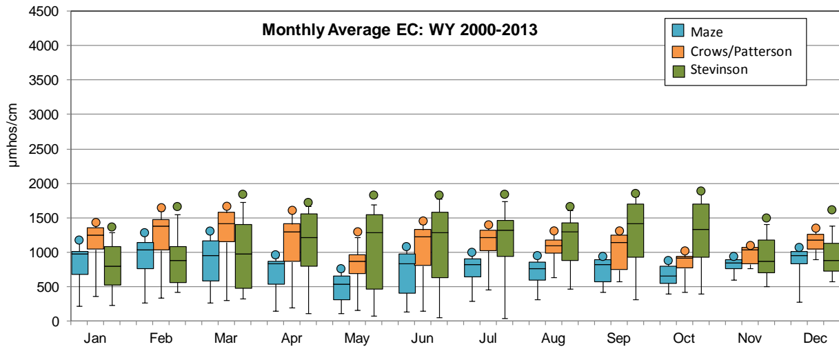
WY 2000 –2013 Monthly average EC by month (Jan, Feb, Mar,...) at Maze, Crows/Patterson, Stevinson
