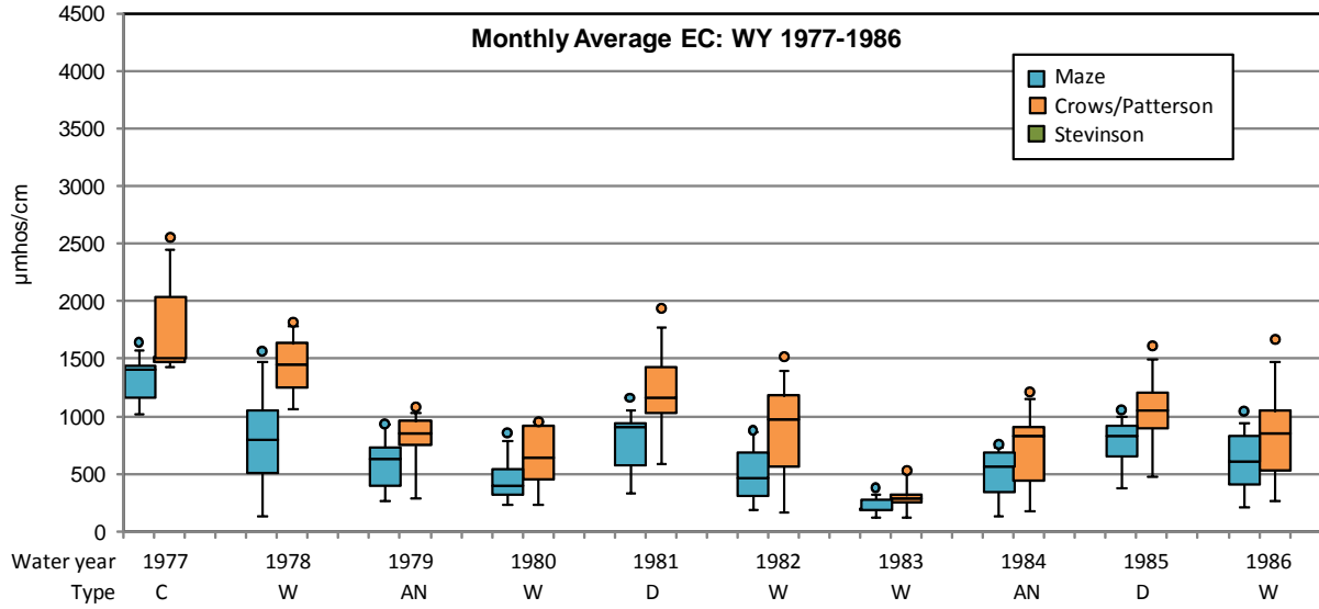
WY 1977 - 1986 Observed monthly average EC at Maze, Crows/Patterson, Stevinson by WY
