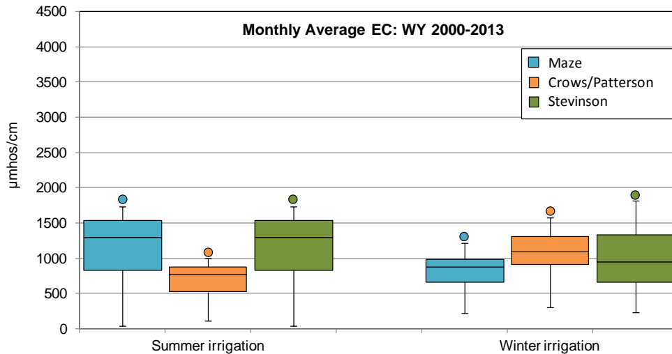
WY 2000-2013 EC at Maze, Crows/Patterson, Stevinson by irrigation season
