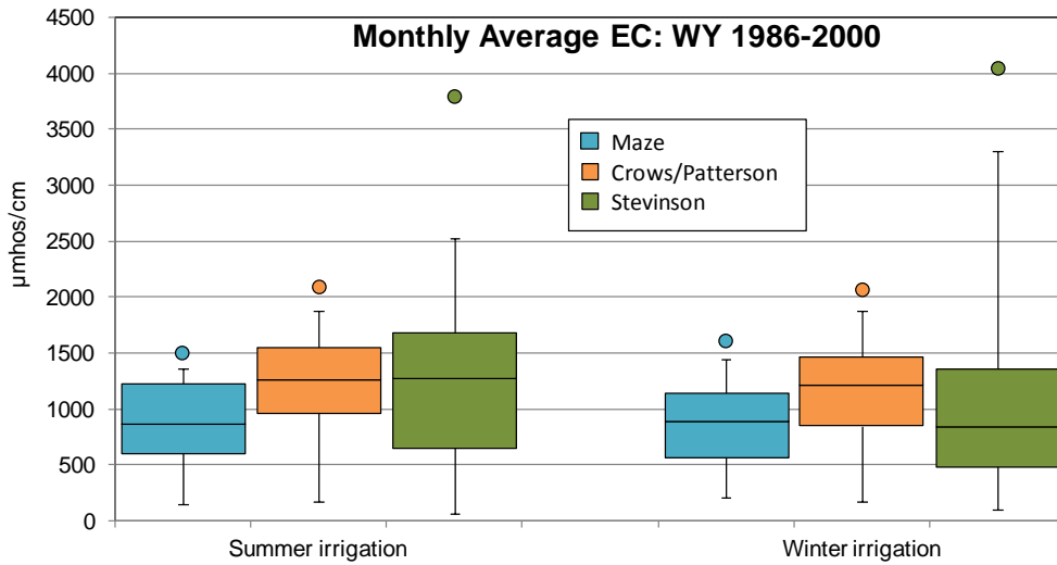
WY 1986-2000 EC at Maze, Crows/Patterson, Stevinson by irrigation season
