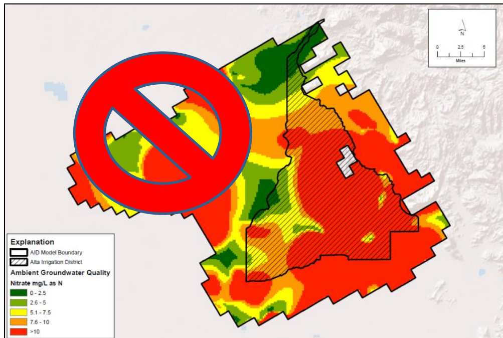
Interpolated Ambient Upper Zone (< 200 feet) Nitrate Concentrations
